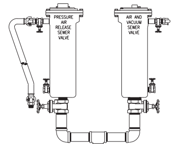
SHOWN WITH OPTIONAL BACKFLUSH ATTACHED
