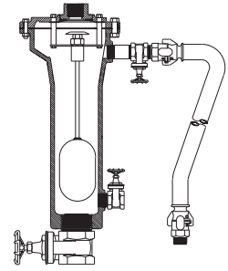
SEWAI ® AIR/VACUUM VALVE SHOWN WITH OPTIONAL BACKFLUSH ATTACHED
