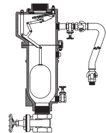
COMBO SEWAI ® SHOWN WITH OPTIONAL BACKFLUSH ATTACHED
