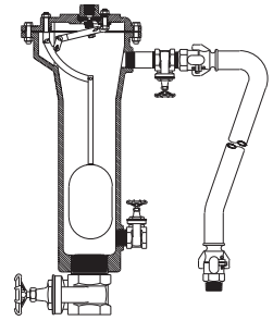
SEWAI ® PRESSURE AIR RELEASE VALVE SHOWN WITH OPTIONAL BACKFLUSH ATTACHED
